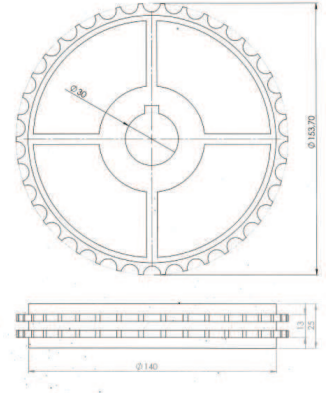
12.7 HASIRBAND DİŞLİ Z.38 Göbek; Ø25mm Ø30mm 40.40 kare
