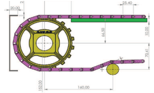
25.4 HASIR BANT DİŞLİ Z.18
